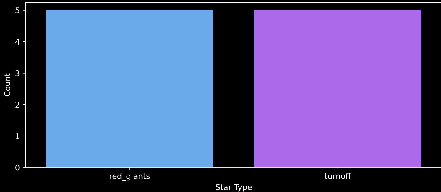
APOGEE DR17 Field: [Bestars] Count plot of Star Type
