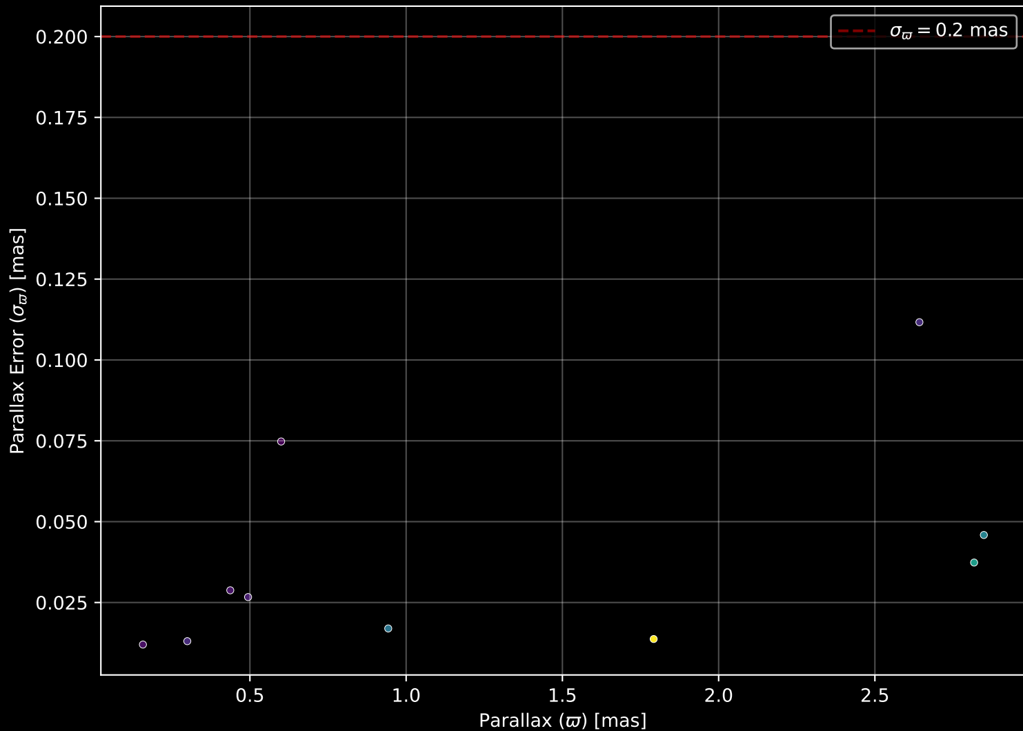
APOGEE DR17 Field: [Bestars] Parallax Quality (n= 10)
