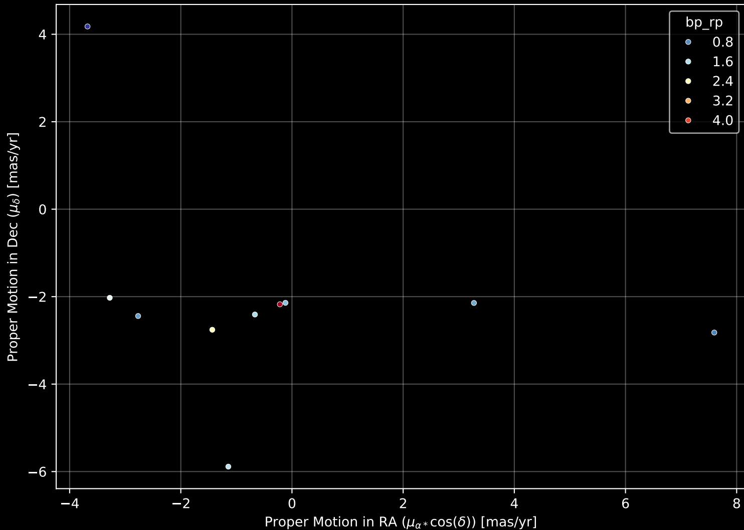
APOGEE DR17 Field: [Bestars] Proper Motion Diagram (n= 10)
