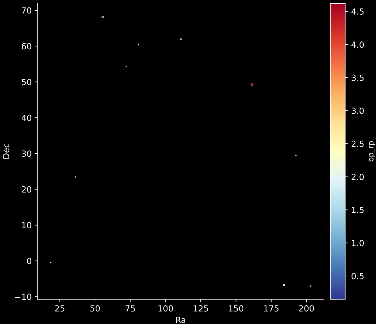
APOGEE DR17 Field: [Bestars] Stars: 10
