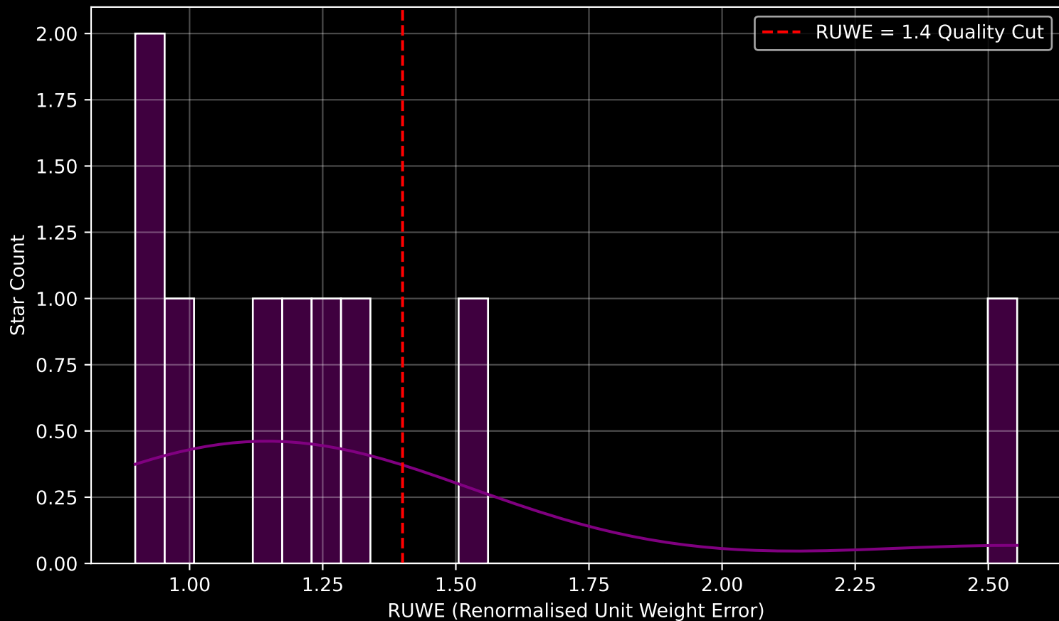
GAPOGEE DR17 Field [Bestars] RUWE Distribution (n= 9)
