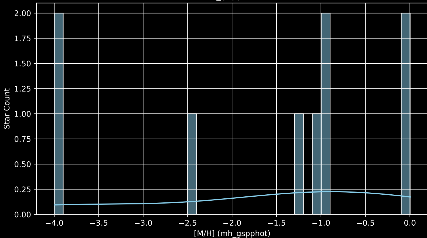
APOGEE DR17 Field: [Beststars [M/H] (mh_gspphot) (n= 9)
